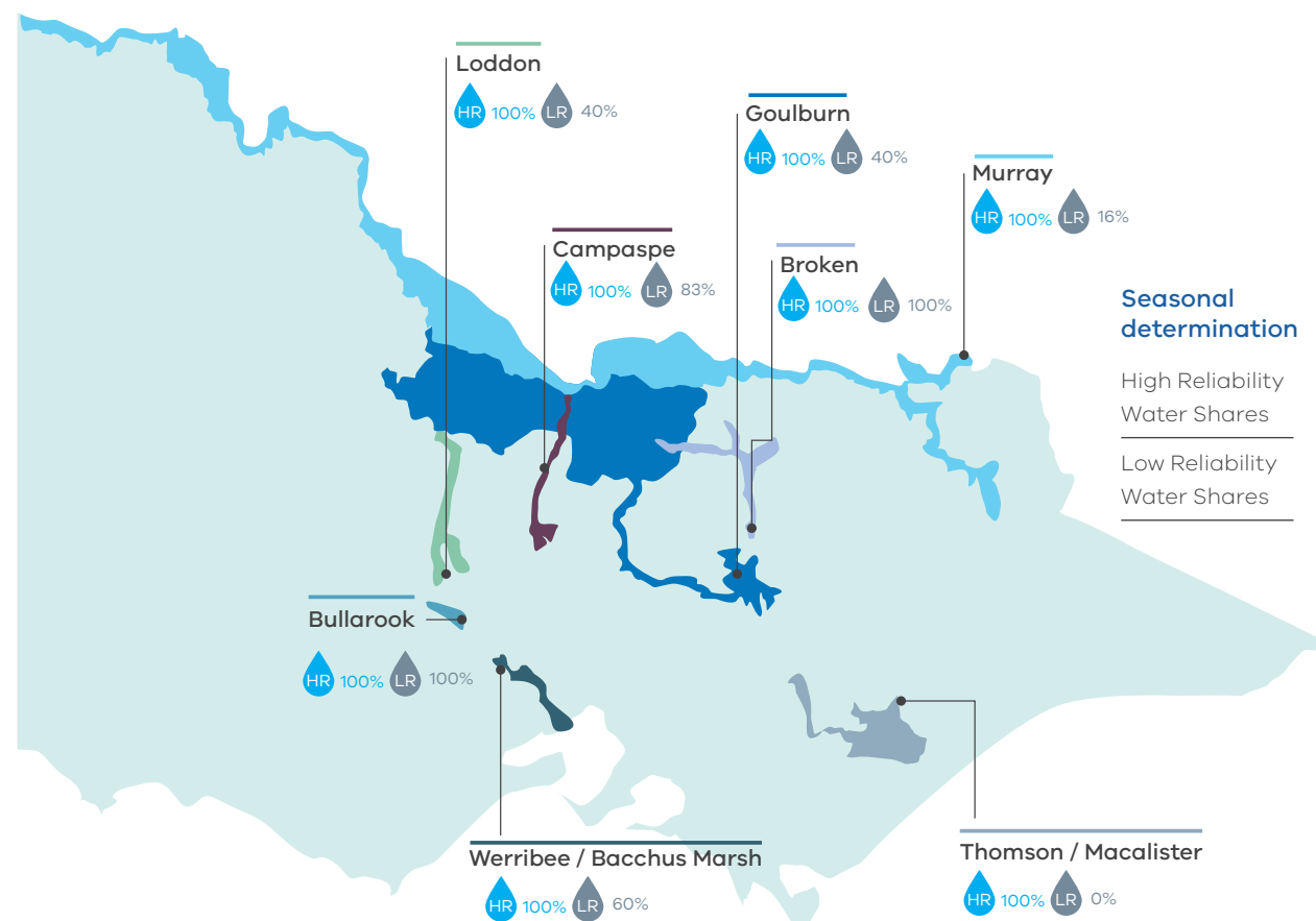
Figure 4. Seasonal determinations in Victorian declared systems as at 1 December 2023
